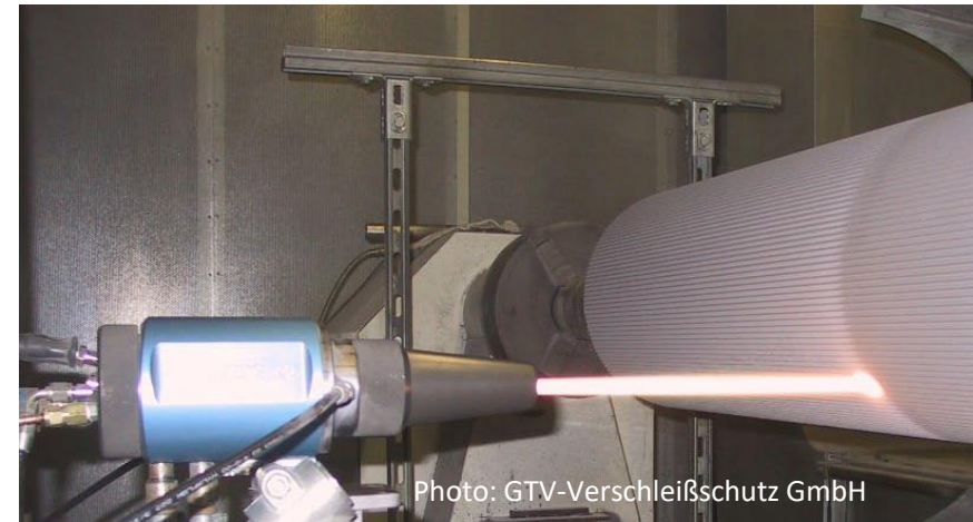
High velocity oxygen fuel spraying (HVOF/HVAF): Equipment
