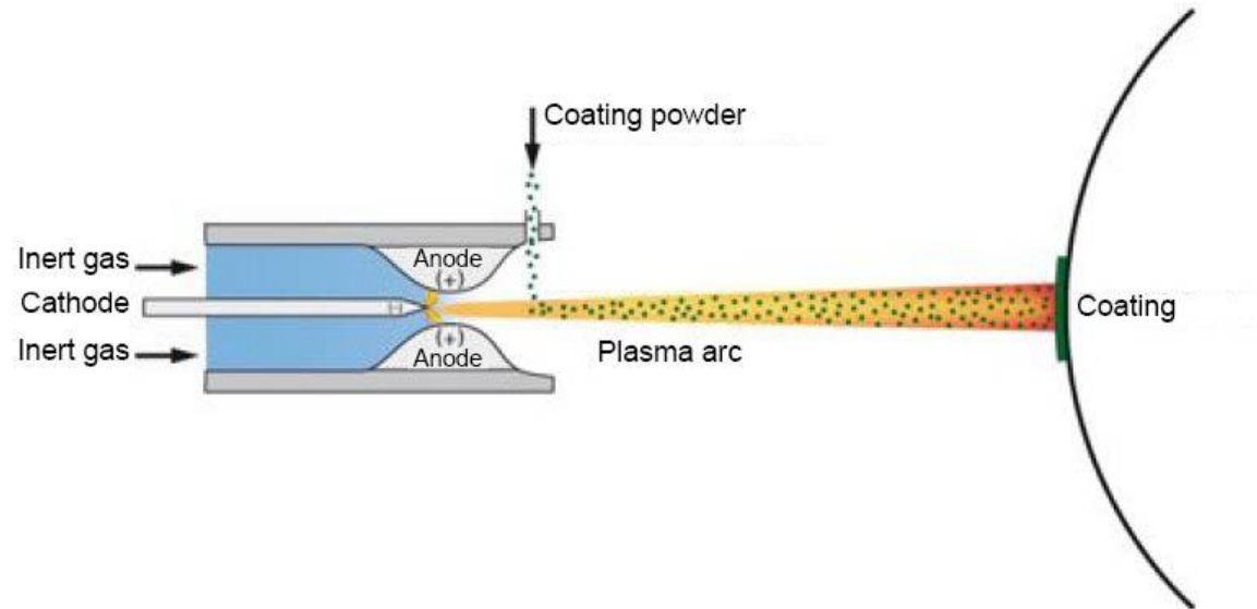
Plasma spraying (APS/VPS/APSS): Technique
