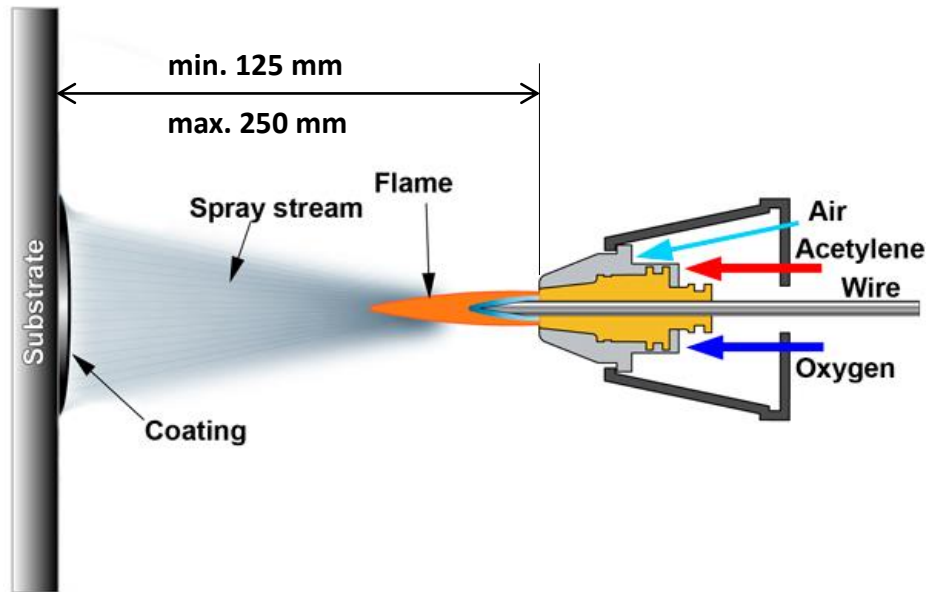
Wire flame spraying (WFS): Technique
