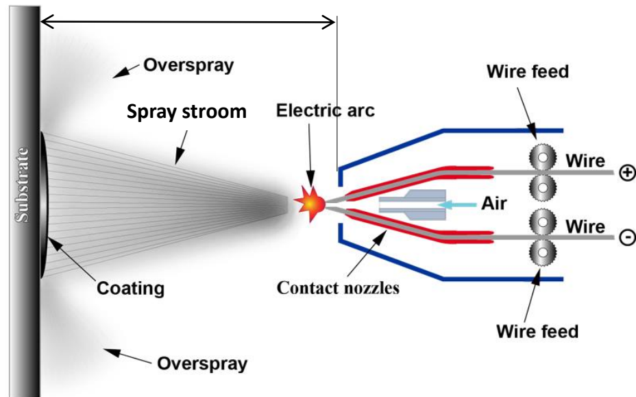
Arc spraying (AS): Technique
